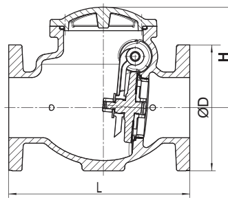
Size 2"-4"
